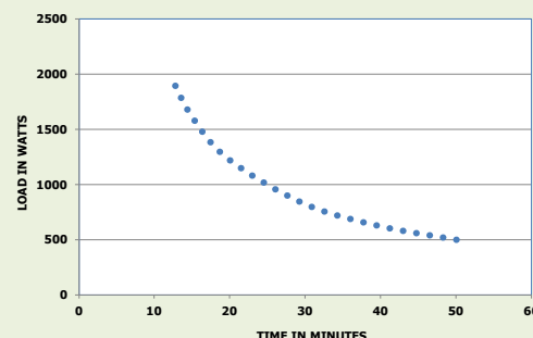
LFP 2500 BATTERY RUN TIME VERSUS POWER (ROOM TEMPERATURE TESTING CONDITIONS)
