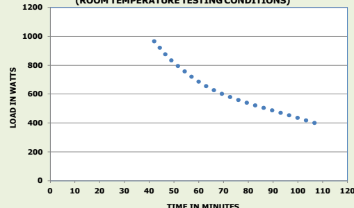
LFP 1251 C3 BATTERY RUN TIME VERSUS LOAD UPS internal battery plus C3 three external batteries (ROOM TEMPERATURE TESTING CONDITIONS)
