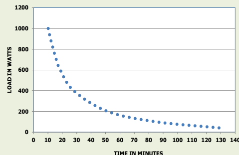
LFP 1251 internal BATTERY RUN TIME VERSUS POWER (ROOM TEMPERATURE TESTING CONDITIONS)
