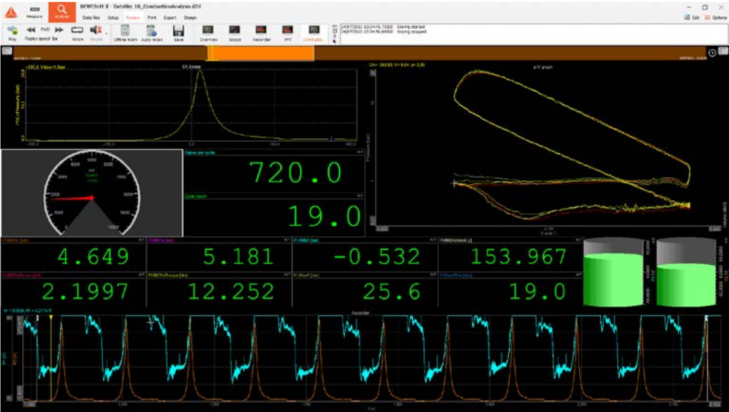
DewesoftX combustion analyzer plug-in, including real-time PV (cylinder pressure/volume) graph
