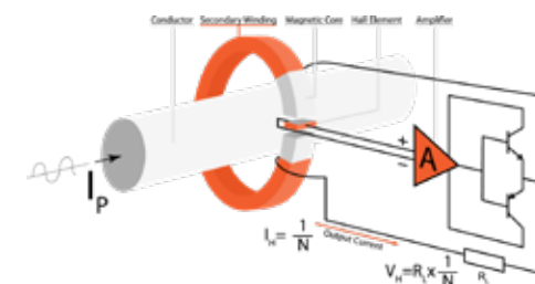
Closed loop current sensor
