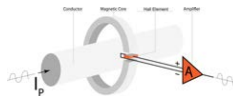
Open loop current sensor
